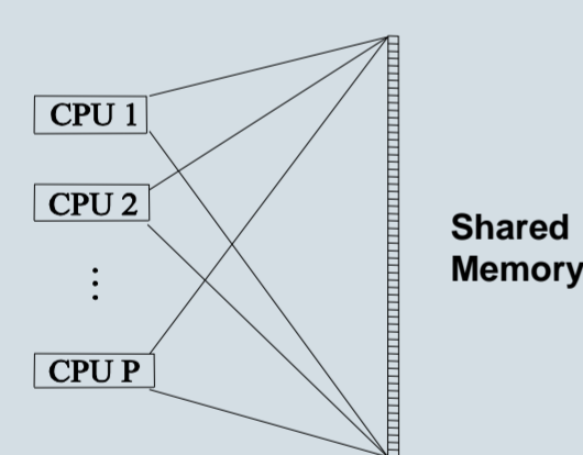
PRAM model
